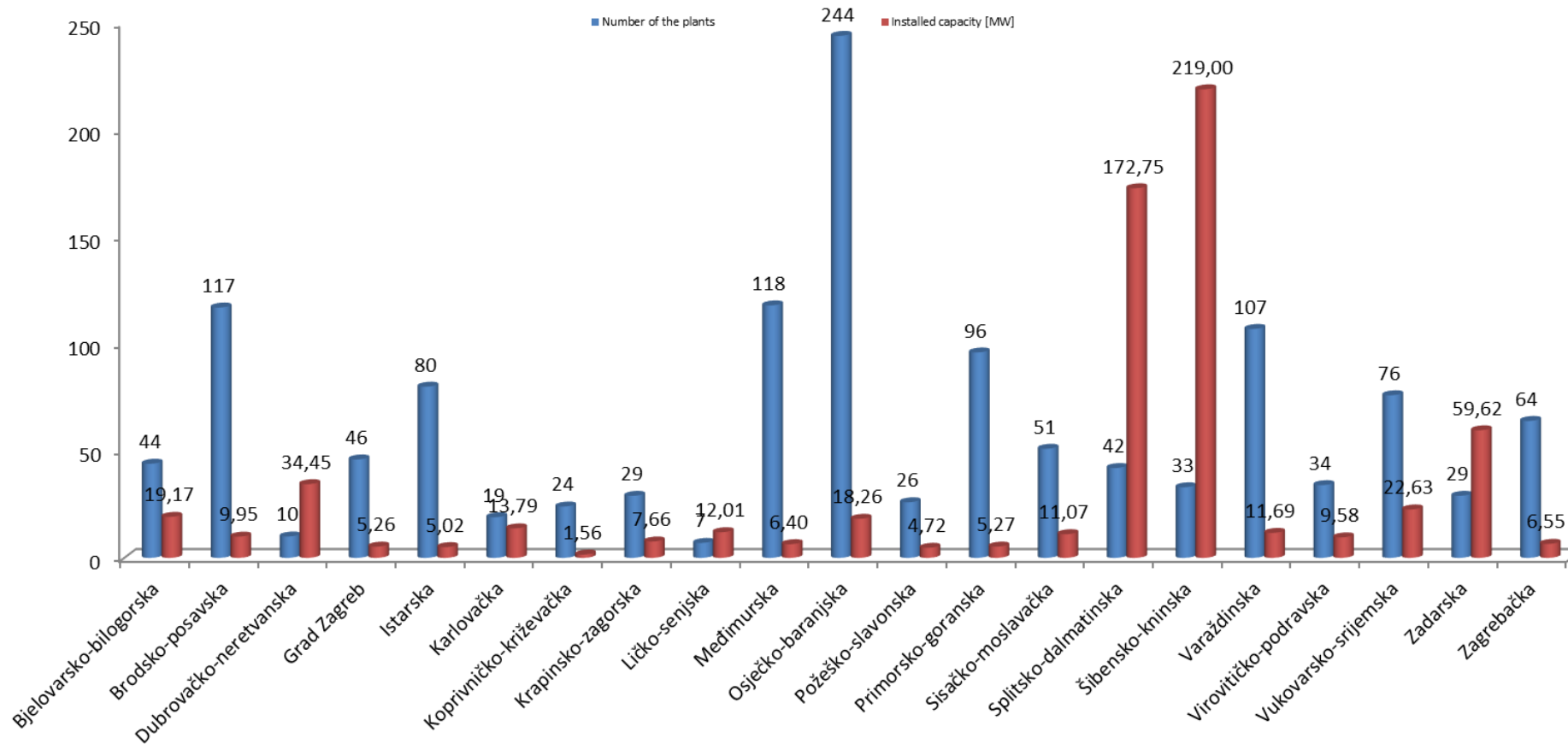
Installed capacity and number of the plants in the incentive system for renewable energy sources per counties
